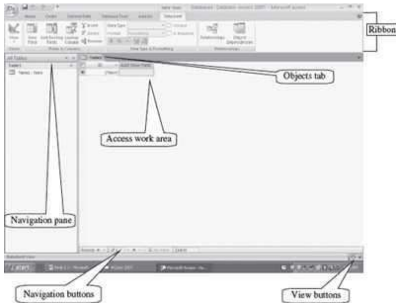
Figure 19.4 MS-Access 2007 screen
