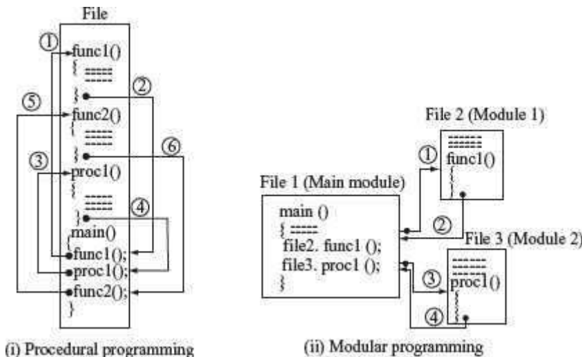
Figure 8.6 Structured programming
