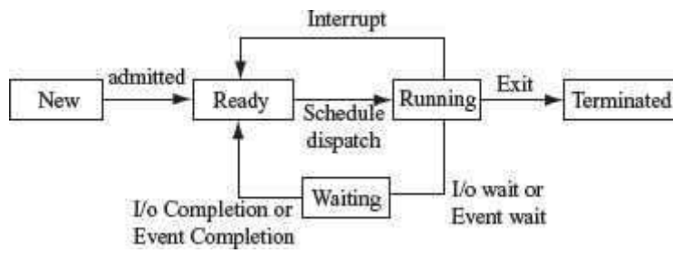
Figure 7.6 Process states
