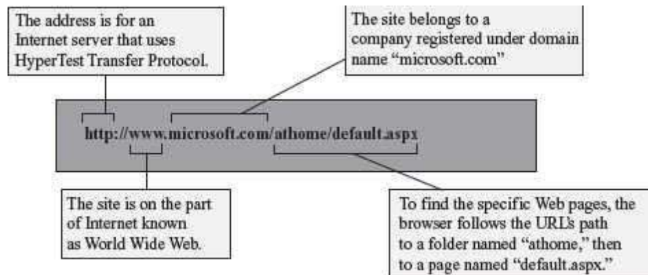
Figure 10.10 An URL
