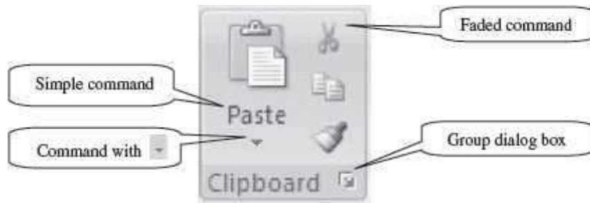
Figure 17.10 Command symbols
