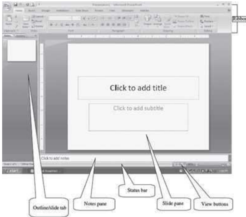
Figure 18.4 MS-PowerPoint Screen
