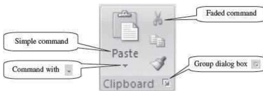
Figure 19.9 Command symbols
