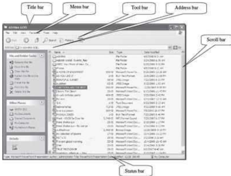
Figure 15.7 A window
