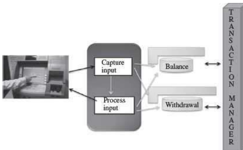
Figure 11.8 Transaction processing
