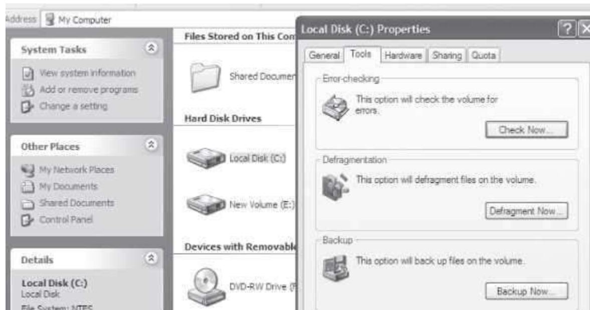
Figure 15.27 The scandisk
